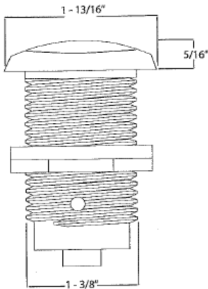
Assembly View
