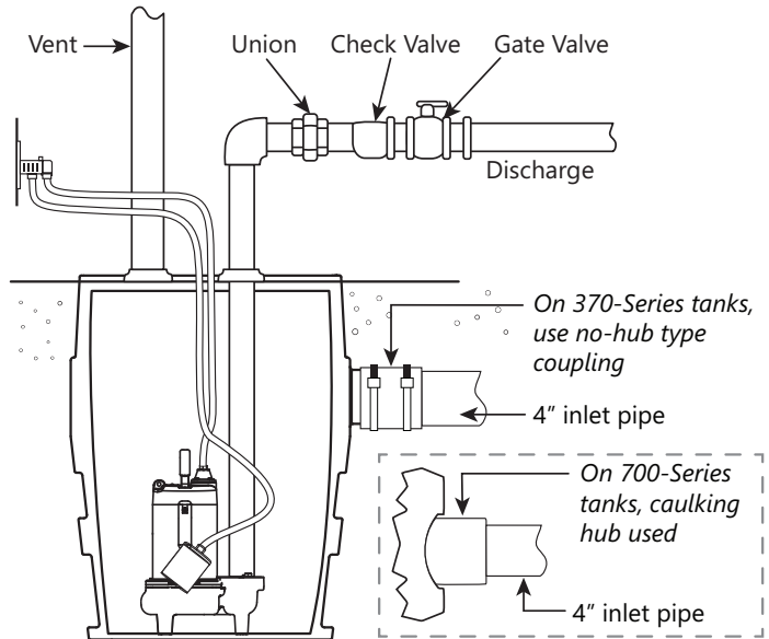
Figure 3. Typical Simplex System Installation (variations may apply)
