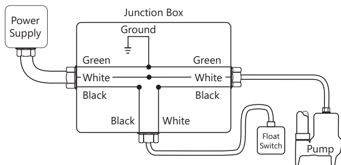
Figure 2. Direct Wiring of 115 V or 208/230 V, 1-Phase, Automatic
