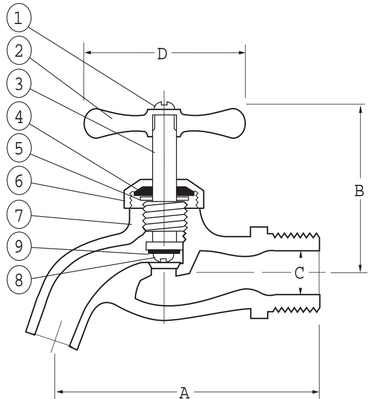
Pictured Model T-532 Cut-away
