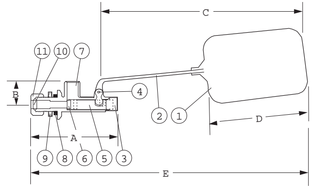
Pictured Model T-35 Cut-away
