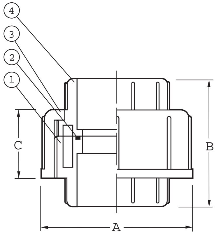
Pictured PVC Schedule 80 Unions Cut-away
