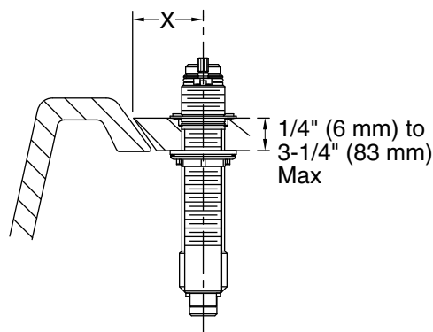
Finished Rim-Mount Installation
