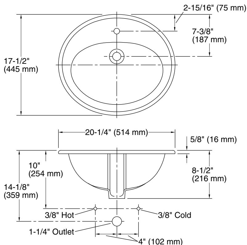
Standard Installation
