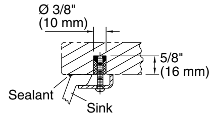
Marble Installation
