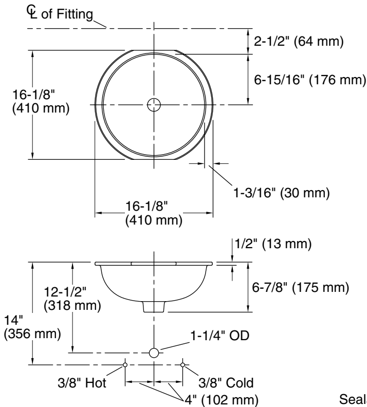
Standard Installation
