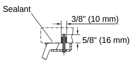
Marble Installation
