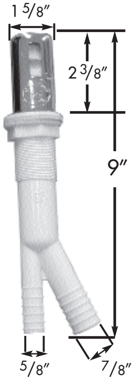
CHROME PLATED AIR GAP
