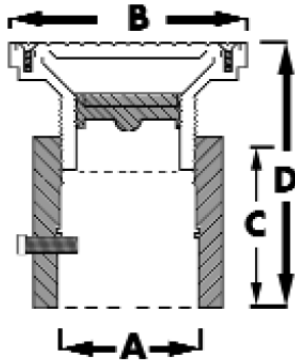
CLEANOUT DIMENSIONS
