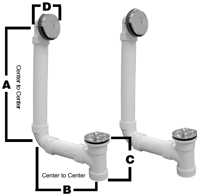
ONE HOLE FACEPLATE
