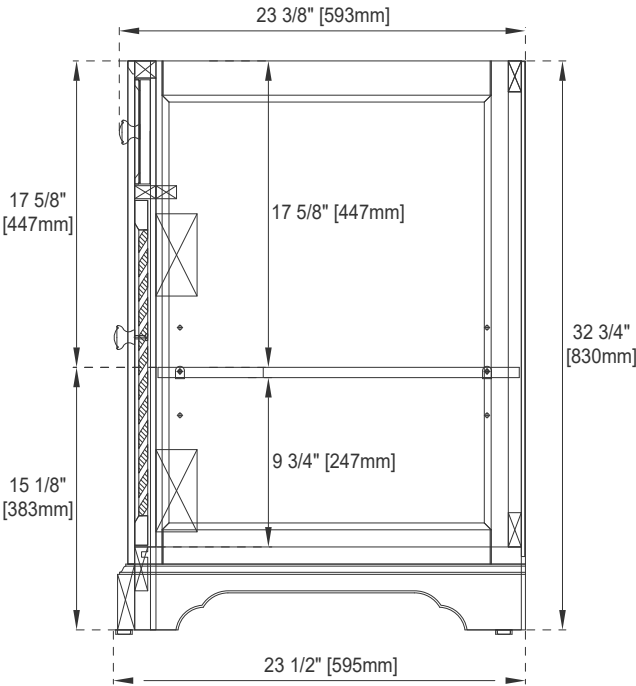
Side View 2
