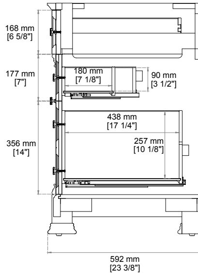
Side View 1
