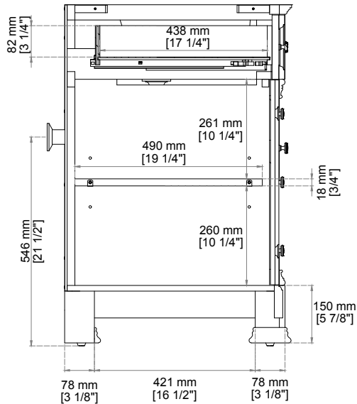
Side View 2
