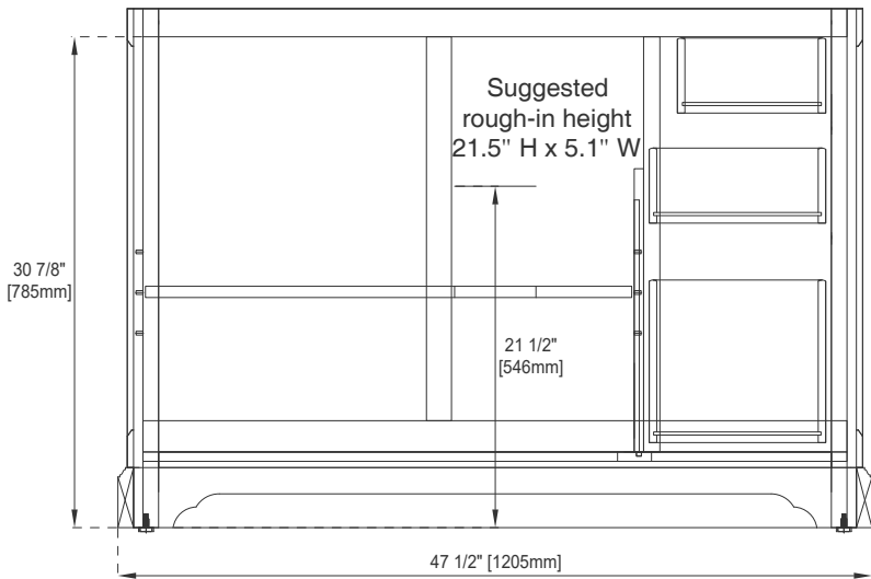
Back View
