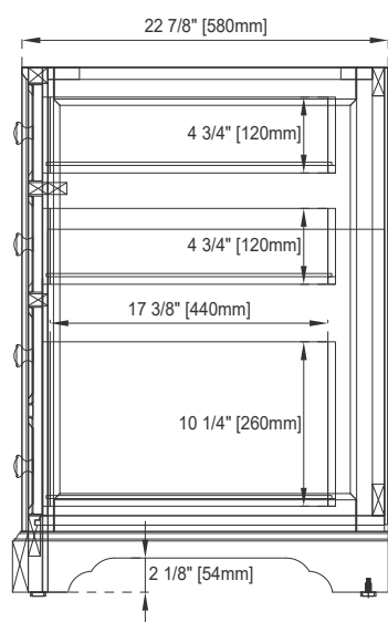
Side View 1
