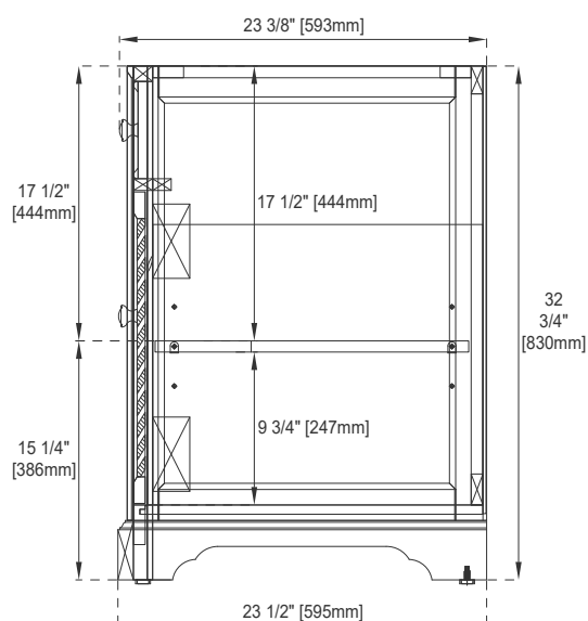
Side View 2
