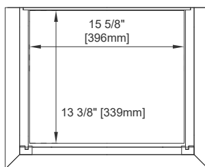
Top View Section C-C
