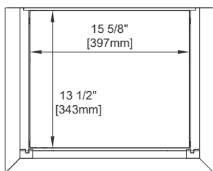
Top View Section A-A
