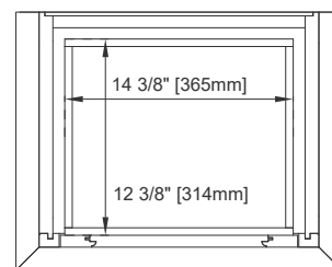
Top View Section B-B
