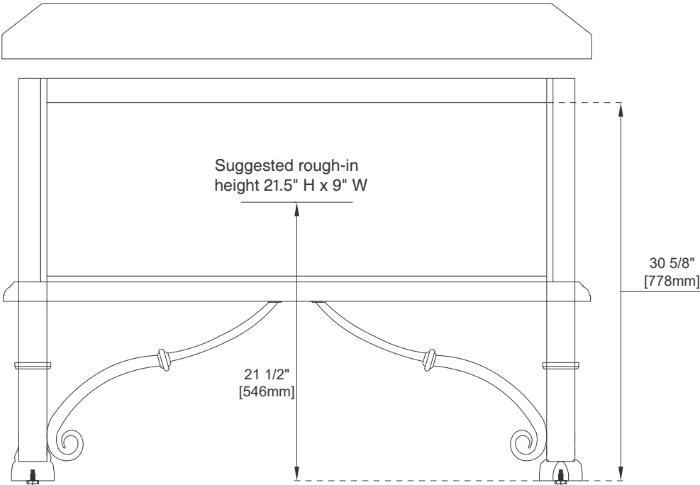
Back View
