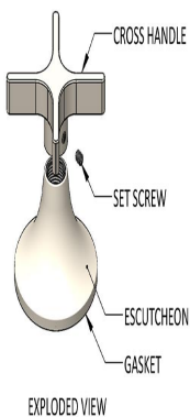
EXPLODED VIEW
