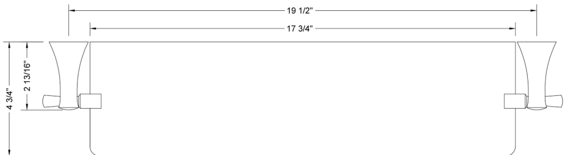
TOP VIEW
