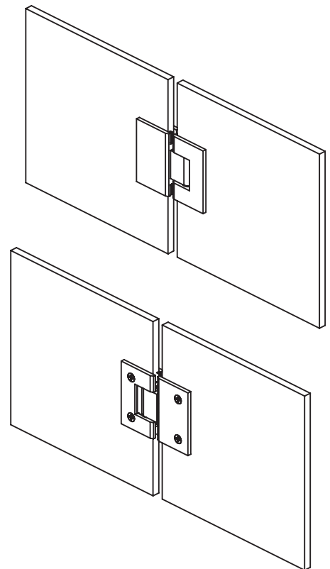
ISO VIEW-3
