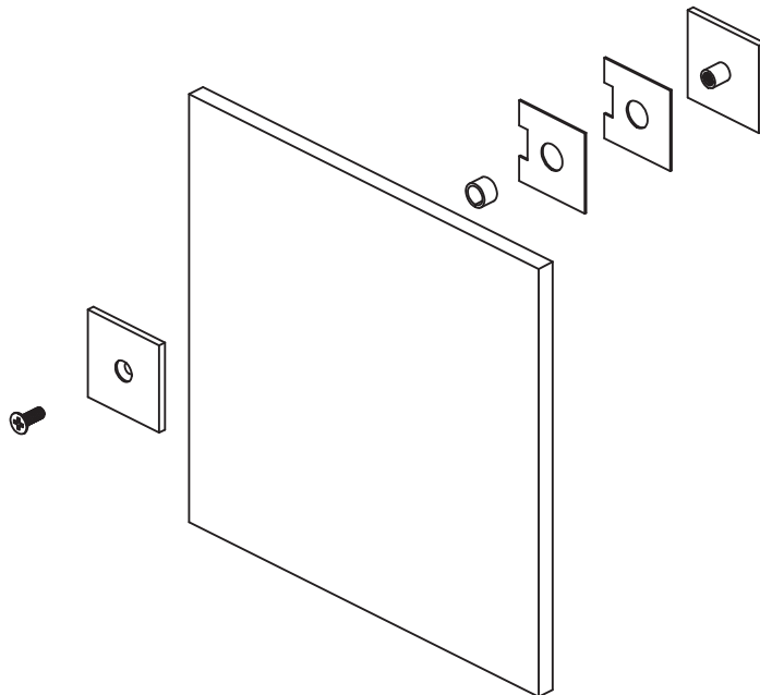
ISO EXPLODED VIEW-2
