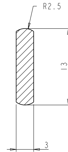
SECTION A-A SCALE 5:2
