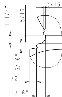
DETAIL B SCALE 3:10
