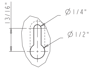
DETAIL A SCALE 3:5
