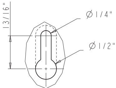
DETAIL A SCALE 7:10
