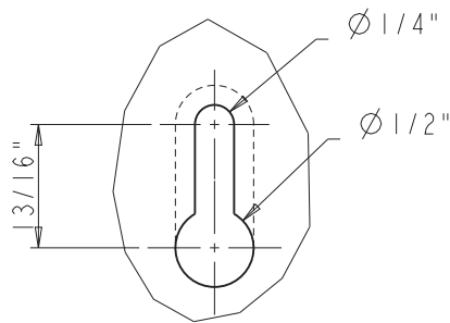
DETAIL A SCALE 3:4
