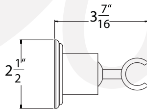
Wall Bracket - P04321xx
