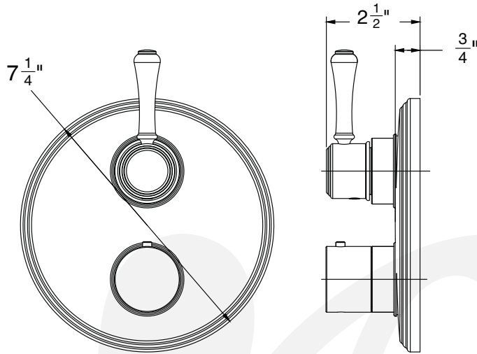
Valve Trim - P27251xx
