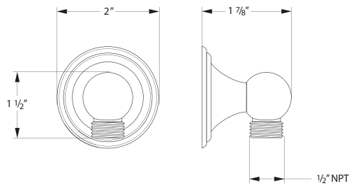
Supply Elbow - P06331xx
