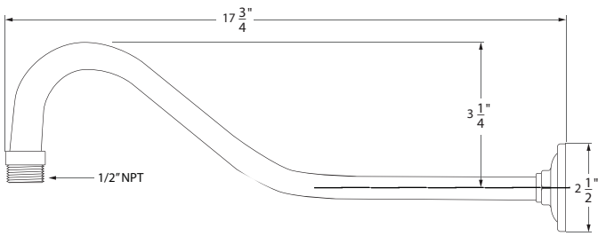
Shower arm - P09281xx
