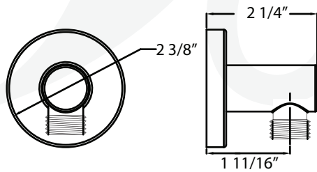
Supply elbow (P10331xx)
