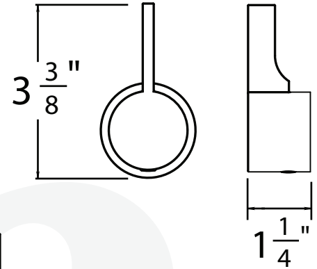
Thermostatic handle (PHB342xx)
