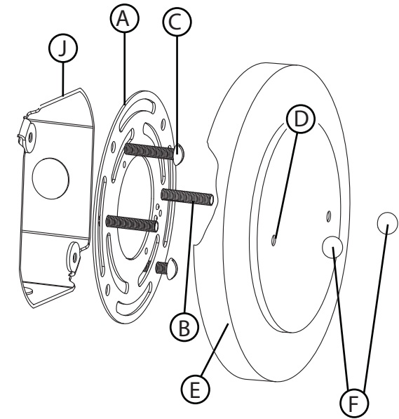
Drawing 1 - Fixture Mounting
