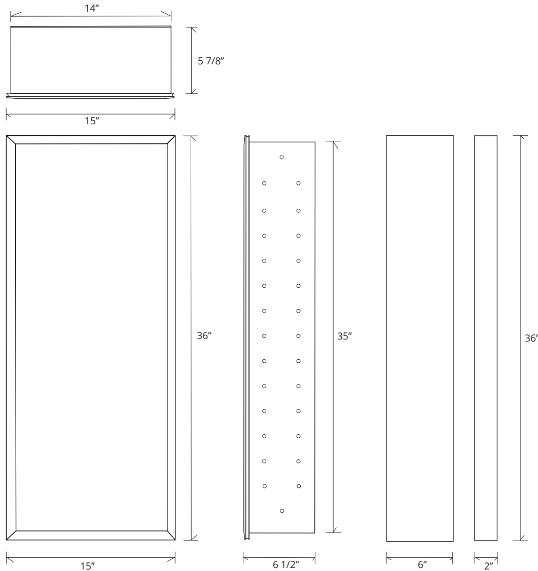
Beveled Mirror Section View
