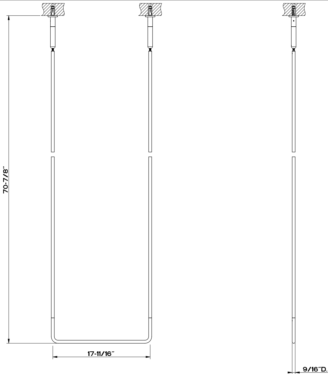
Drywall with rawl plug KD8 installation ( kit 29724 to be ordered apart )
