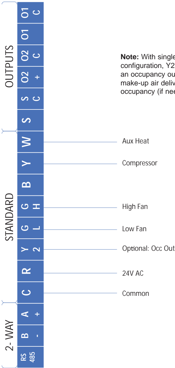
Diagram 4: Standard Communication Wiring (1 Heat / 1 Cool)
