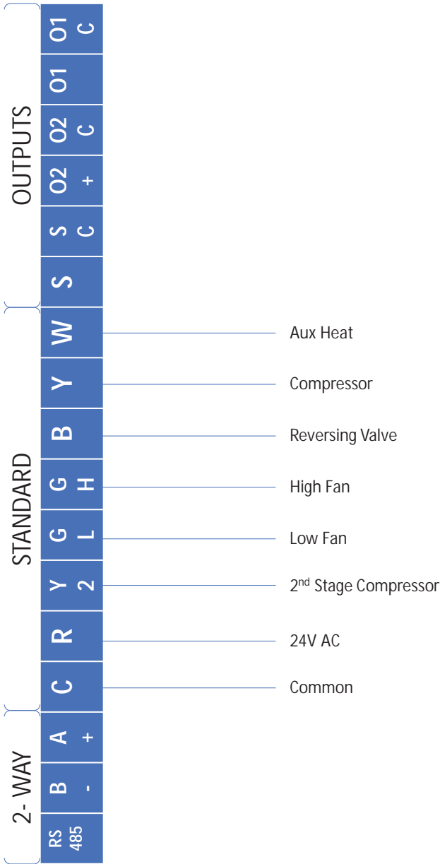
Diagram 2: Standard Communication Wiring (3 Heat / 2 Cool), Factory Default
