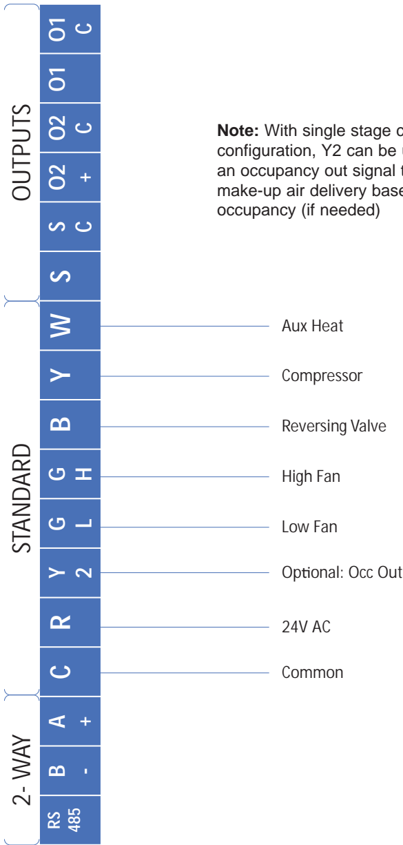
Diagram 3: Standard Communication Wiring (2 Heat / 1 Cool)
