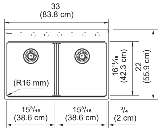
Dimensional Drawing
