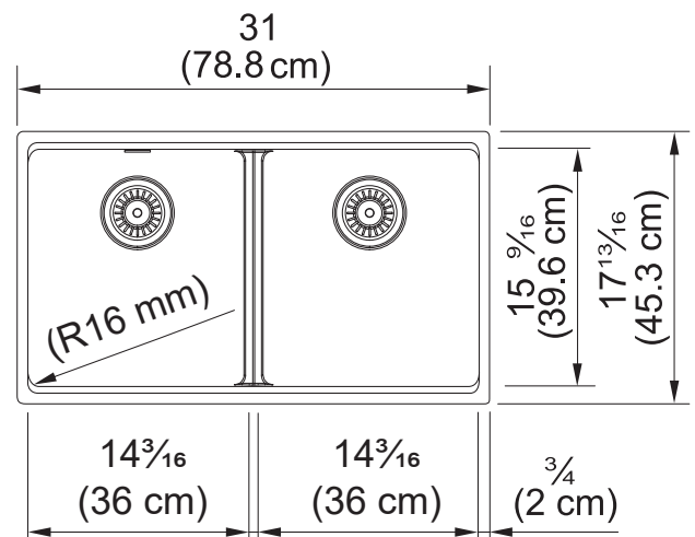
Dimensional Drawing
