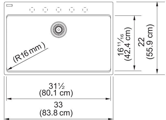
Dimensional Drawing
