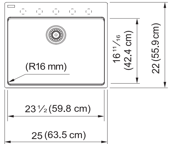
Dimensional Drawing
