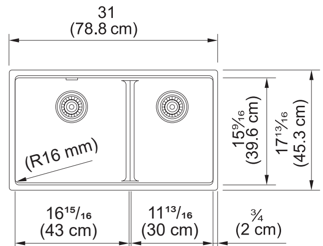
Dimensional Drawing
