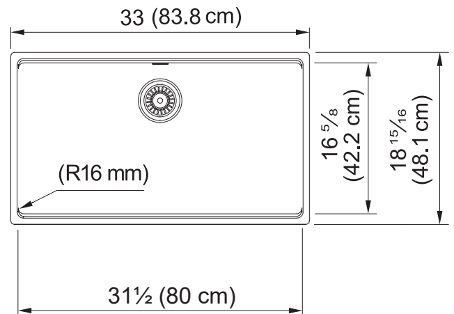
Dimensional Drawing
