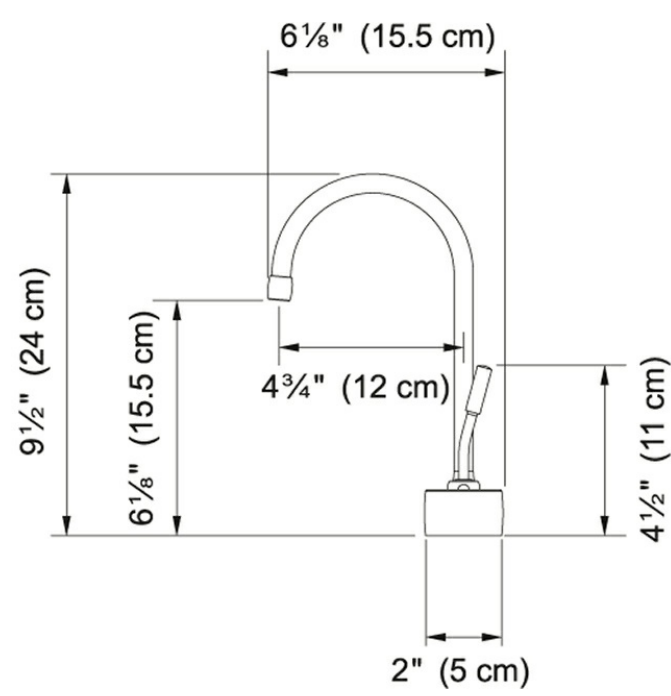
Technical Drawing
