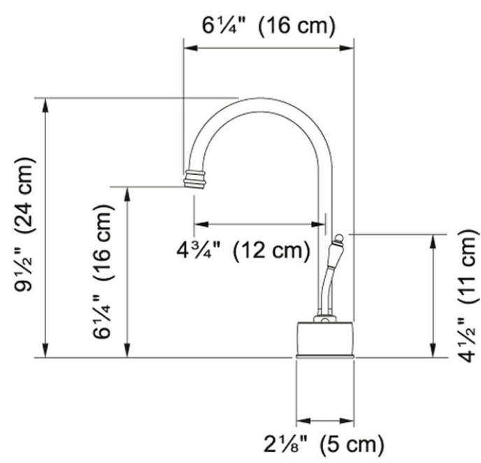
Technical Drawing
