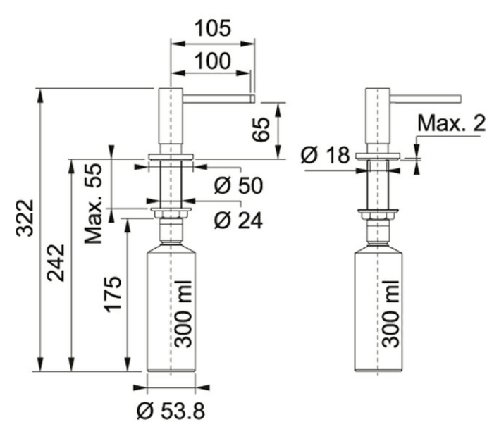
Technical Drawing
