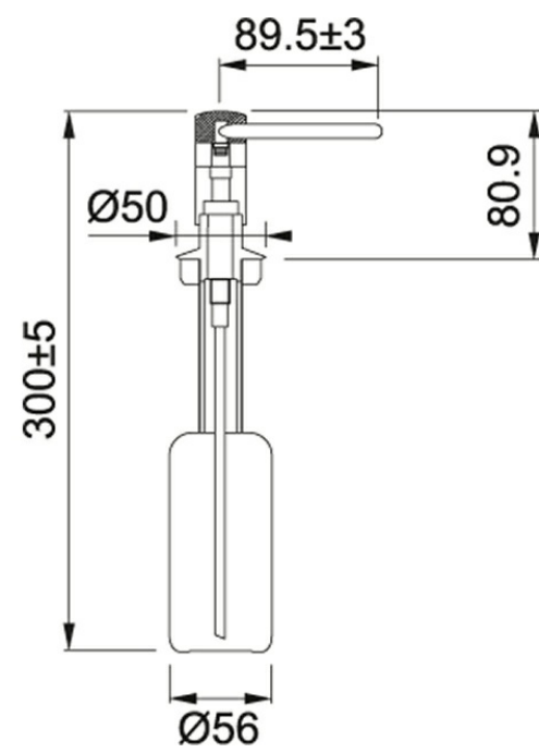
Technical Drawing
