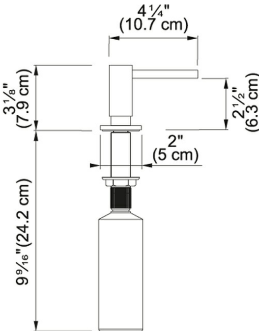
Technical Drawing
