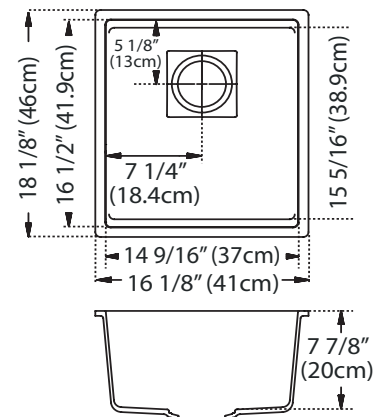
Dimensional Drawing
