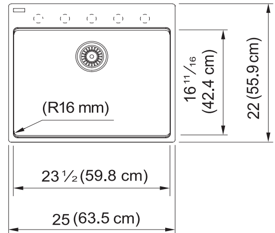
Dimensional Drawing
