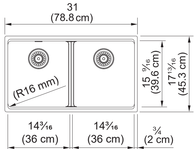
Dimensional Drawing
