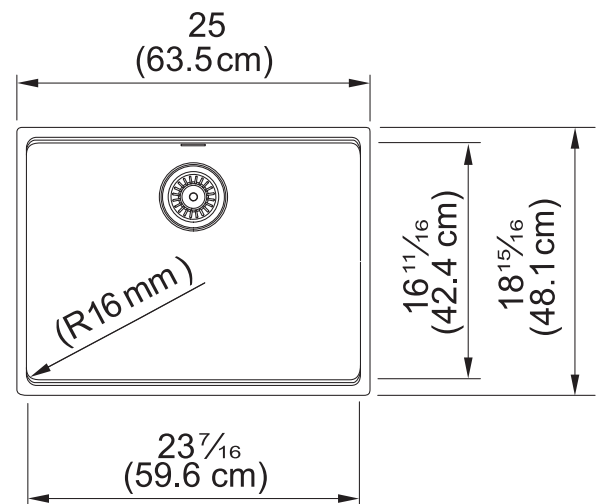
Dimensional Drawing
