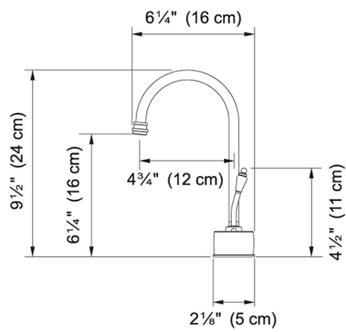
Technical Drawing
