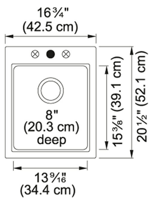
Technical Drawing
