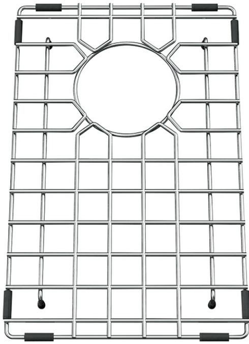
Technical Drawing
